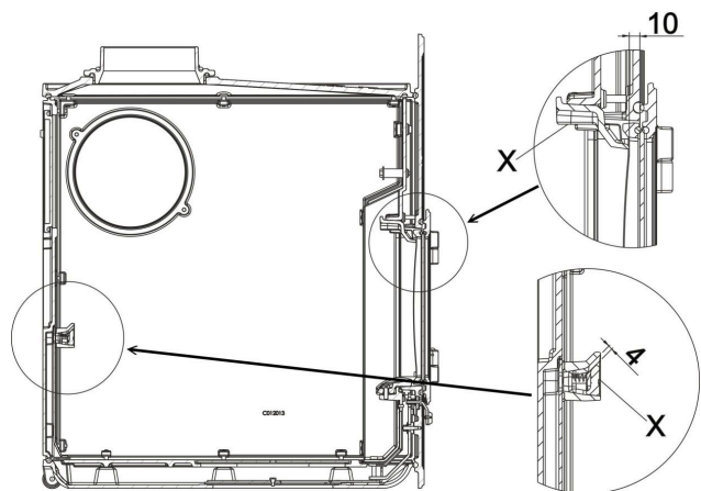
Im. 5: Combustion air setting
