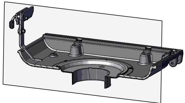
Detail: Air connection piece fitted:
