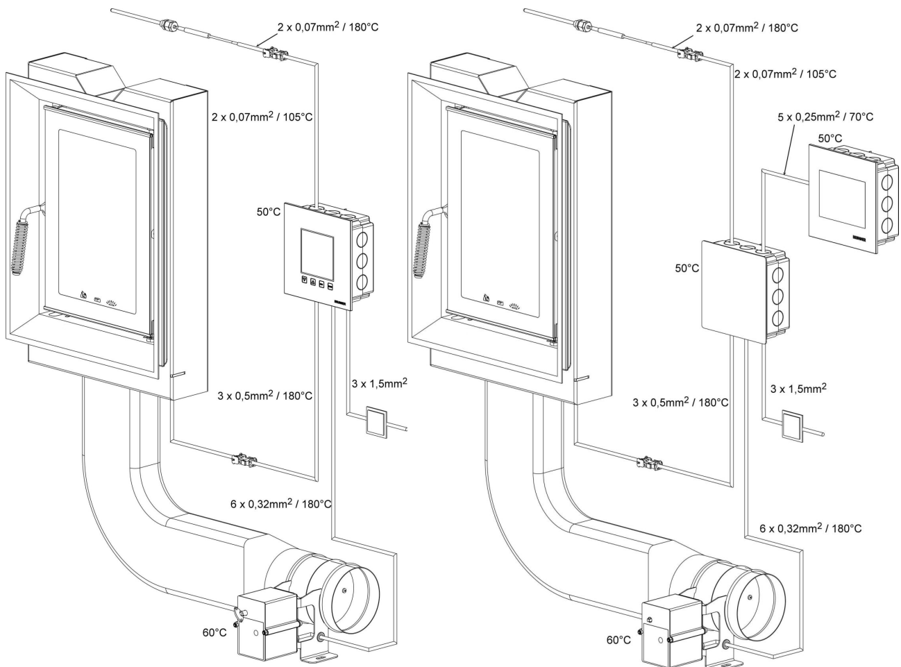
Im. 6: Schematic layout of EAS
