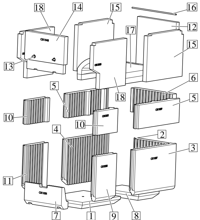
Im. 2: Components
